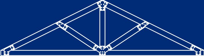
King Truss + Webs
