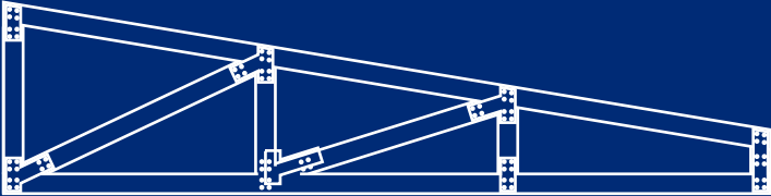
Mono Truss
